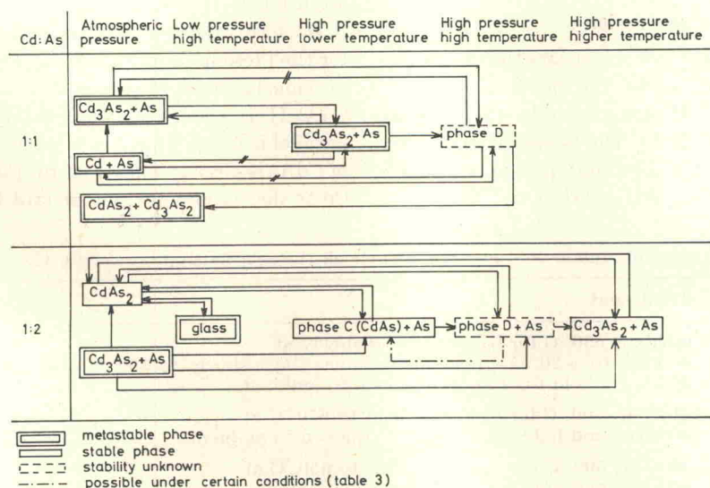
Fig. 6. Stability relationships between phases obtained from high pressures and high temperatures in the \text{Cd}_3\text{As}_2 -As system.
